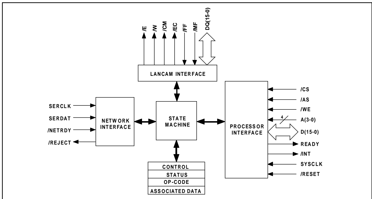
Block Diagram
